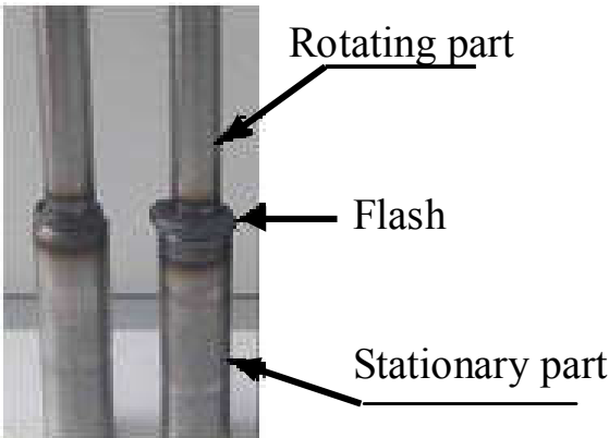
Fig. 2. Friction welded specimens
