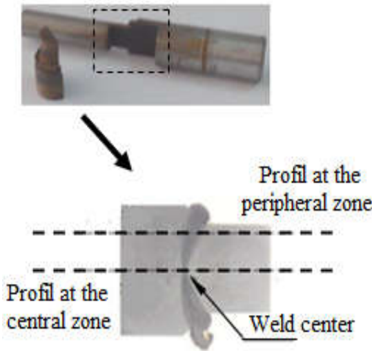
Fig. 3. Hardness test orientation
