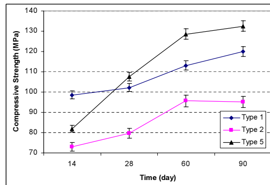
Fig. 9. Compressive strength versus time for mixtures with 5% gypsum replacement
