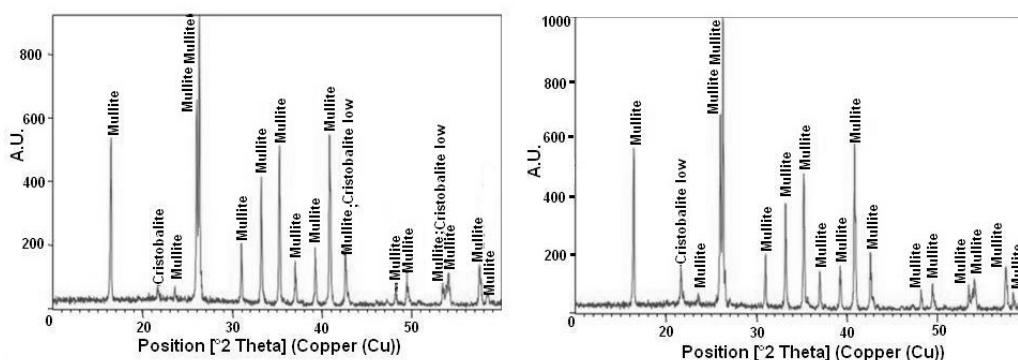
Fig. 8. (a) XRD of the bricks made from feed samples
