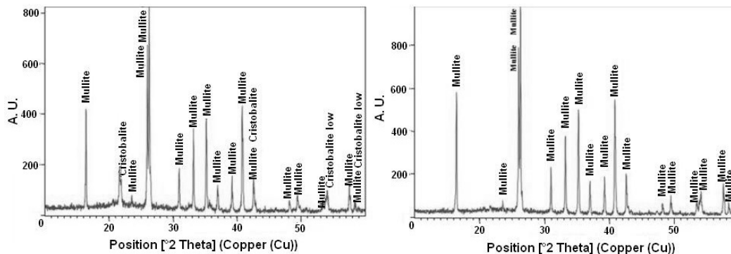
Fig. 8. (b) XRD of the bricks made from underflow samples
