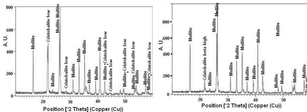
Fig. 8. (c) XRD of the bricks made from overflow samples
