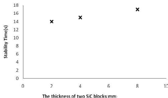
Fig. 16. Stability time at different SiC block sizes.
