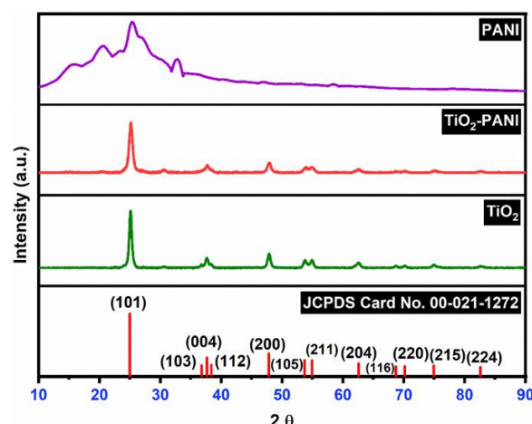
Fig. 3. XRD spectrum of the bare \text{TiO}_2 and \text{TiO}_2 -PANI nanocomposite
