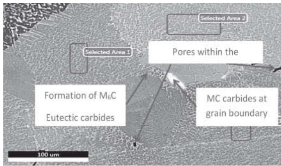
Fig. 21. Sectioned base
